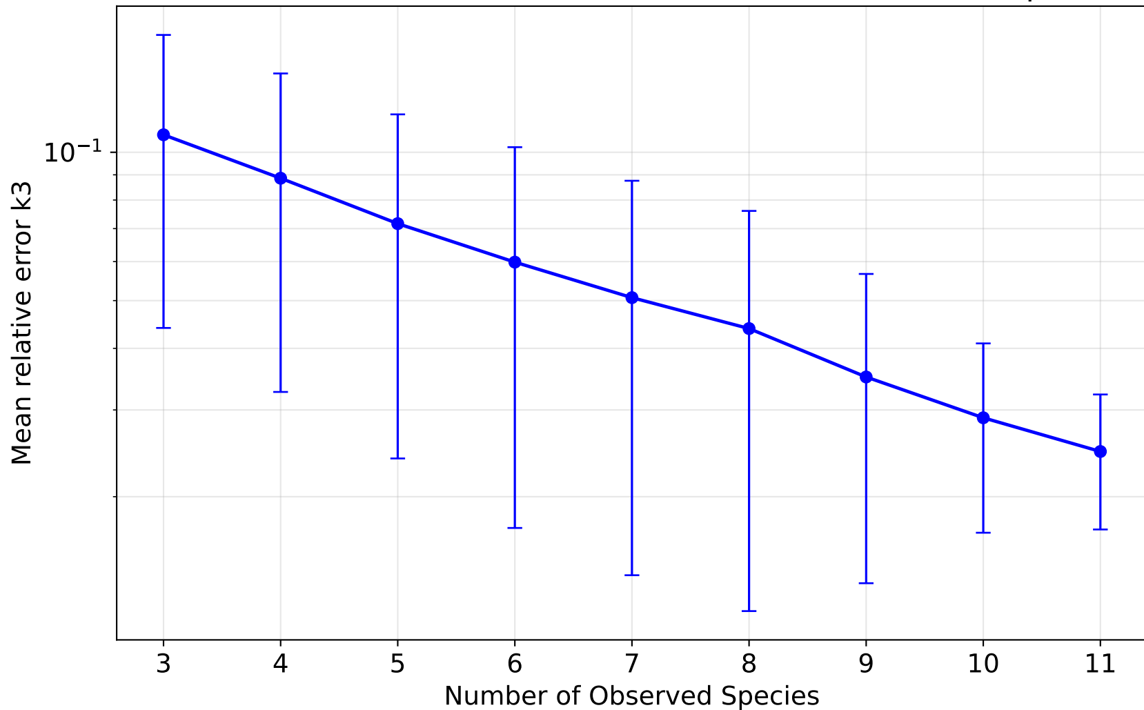
30, 30 — Mean relative error k3 vs number of observed species
